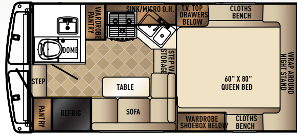
1 TON TRUCK W/ 6'6" OR 8' BED
